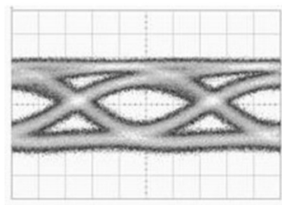
Eye Diagram
