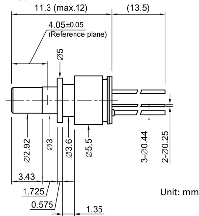
ROSA type
