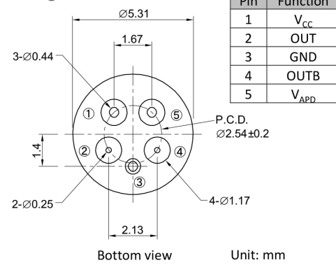
Pin assignment
