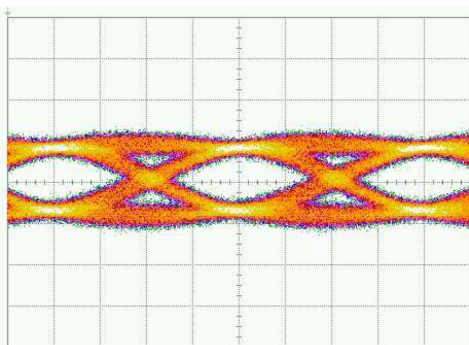
Eye Diagram
