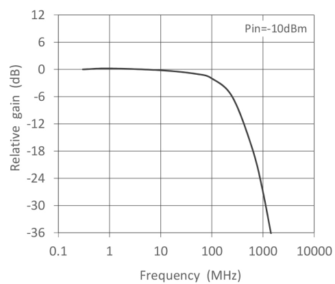
Frequency Response
