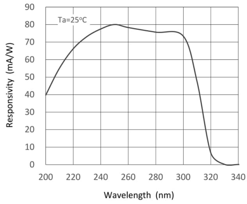
Spectral Responsivity
