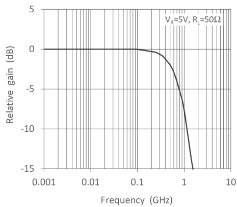
Frequency Response
