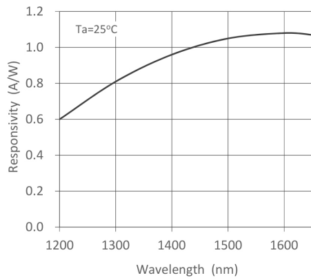
Spectral Responsivity
