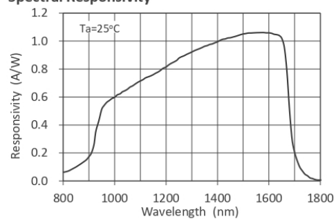
Spectral Responsivity
