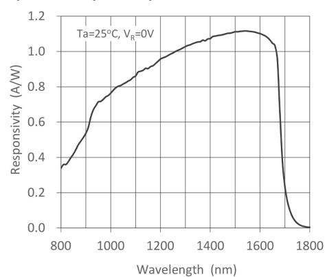
Spectral Responsivity
