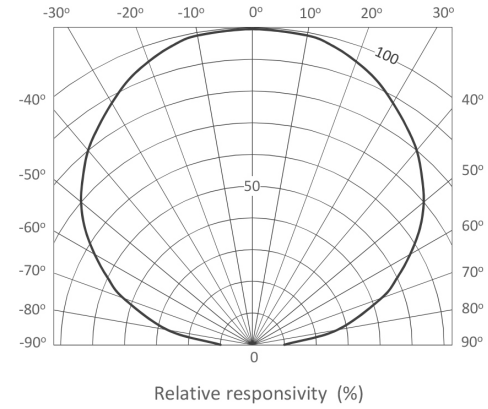
Directivity
