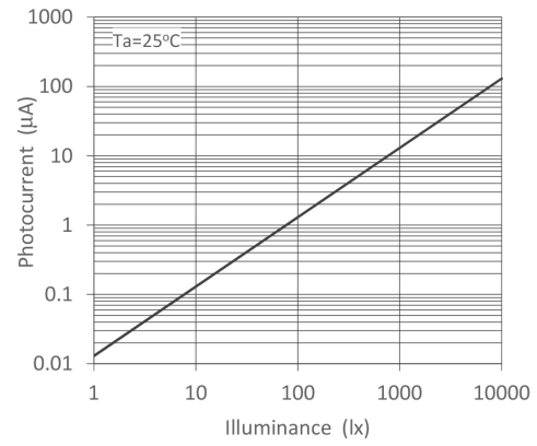
Photocurrent - Illuminance
