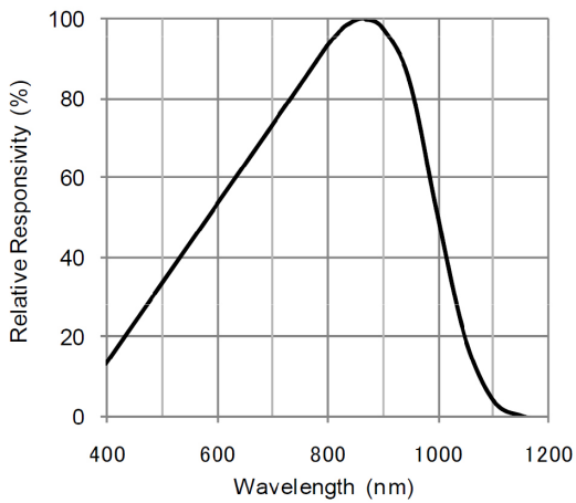
Spectral Responsivity
