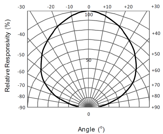
Directivity
