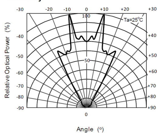
Directivity
