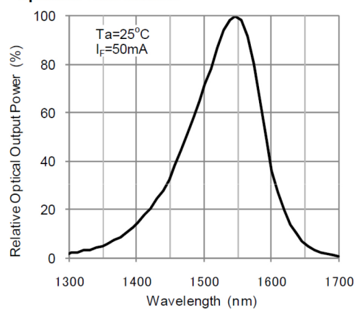
Spectral Distribution
