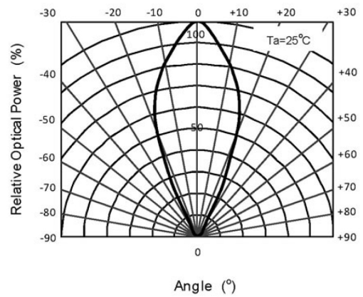
Directivity
