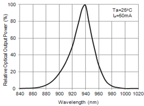
Spectral Distribution
