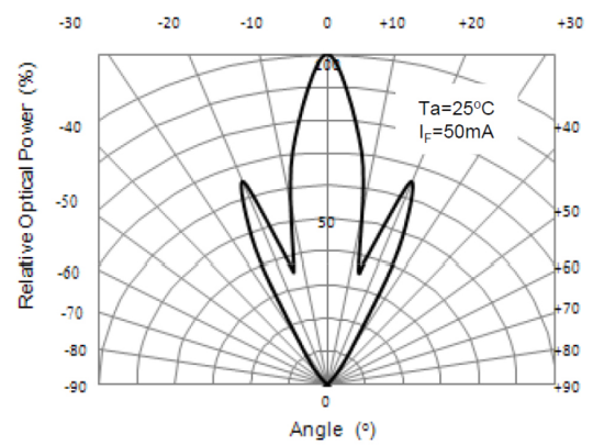
Directivity
