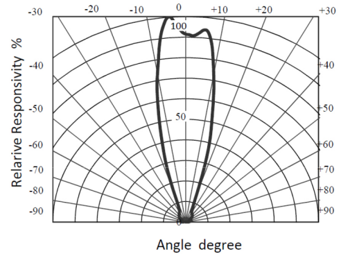
Directivity (Ta=25°C)
