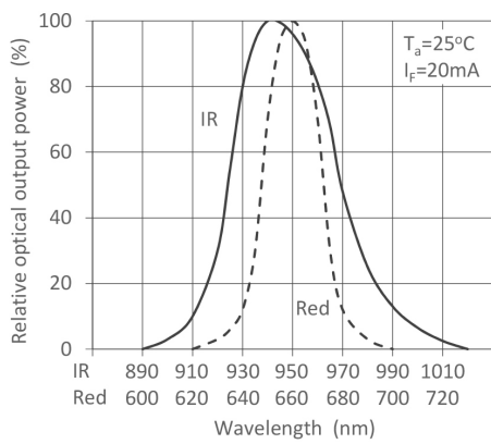
Spectral Distribution
