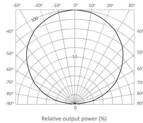
Directivity
