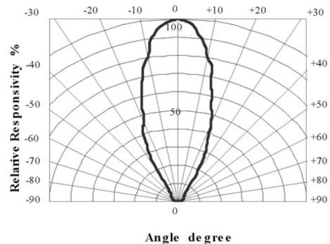
Directivity (Ta=25°C)
