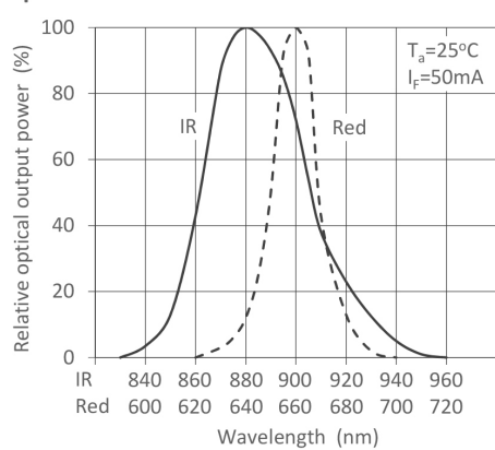
Spectral Distribution
