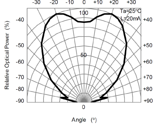
Directivity
