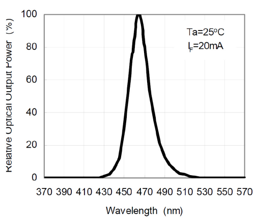
Spectral Distribution
