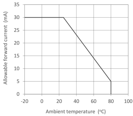
Allowable Forward Current-Ambient Temperature
