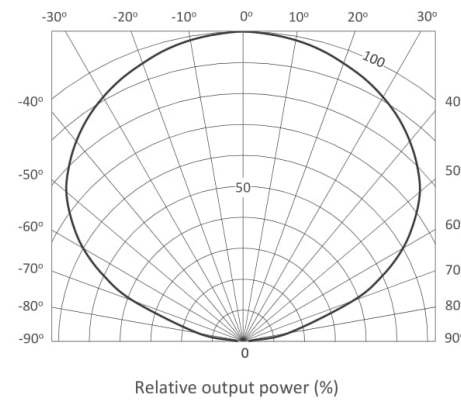
Directivity
