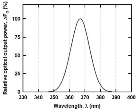
Spectral Distribution (Ta=25°C, I_F=20mA)
