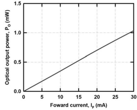
Optical Output Power – Forward Current (Ta=25°C)
