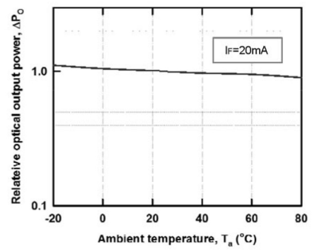
Relative Optical Output Power – Ambient Temperature
