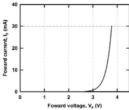
Forward Current – Forward Voltage (Ta=25°C)
