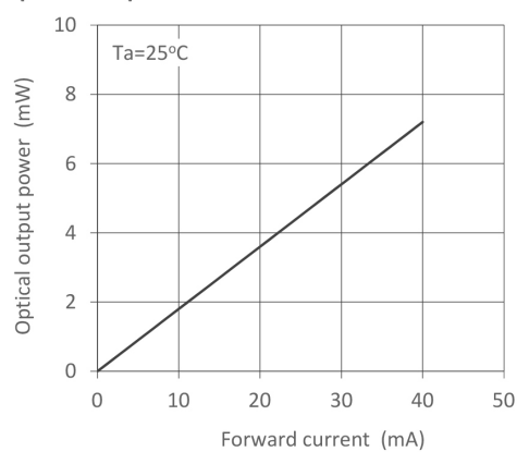
Optical Output Power - Forward Current
