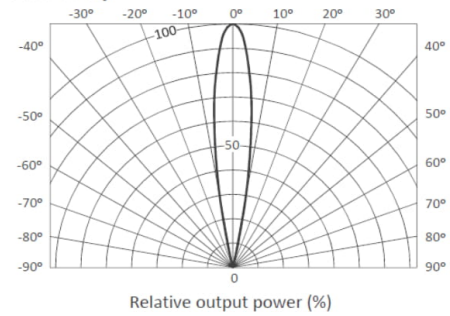
Directivity
