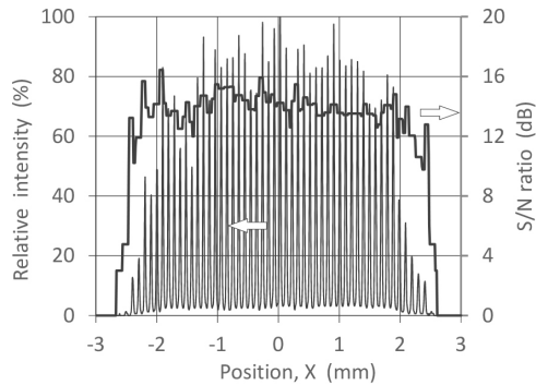
Beam Parallelism
