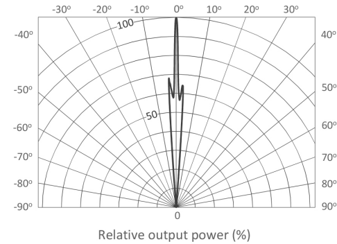
Directivity
